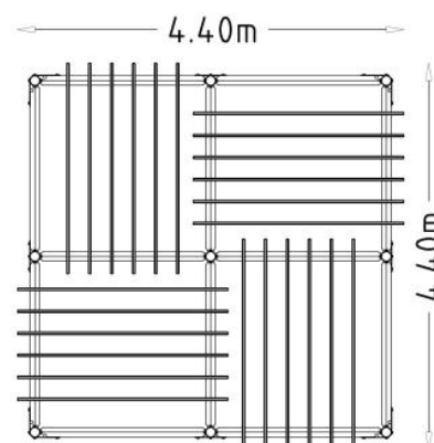
Pergola 4 Sections
